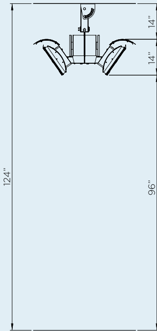
CEILING POLE CLEARANCE WITH HEAT DEFLECTOR
