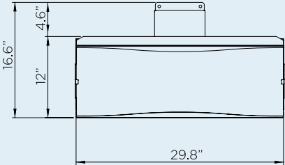
PRODUCT MEASUREMENTS 500 SERIES
