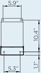
BRACKET MEASUREMENTS
