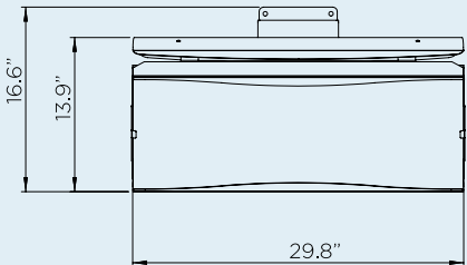
PRODUCT MEASUREMENTS WITH HEAT DEFLECTOR 500 SERIES
