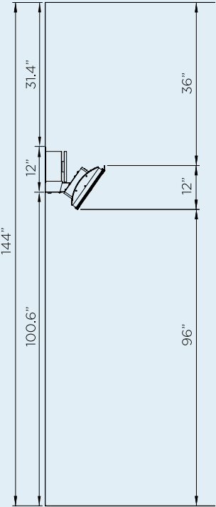
WALL MOUNT CLEARANCE
