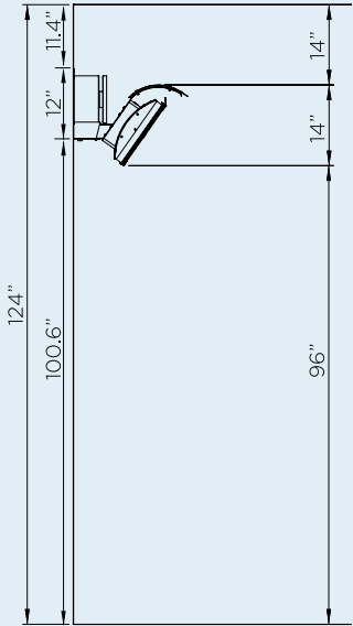
WALL MOUNT CLEARANCE WITH HEAT DEFLECTOR
